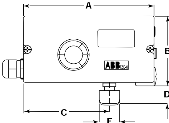
DIMENSIONS 1 inches (mm) AND WEIGHTS pounds (kg)
