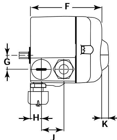
DIMENSIONS 1 inches (mm) AND WEIGHTS pounds (kg)
